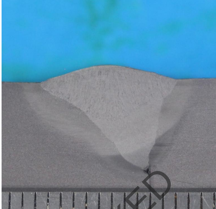
Image 1 of 1 - Macro Specimen 1 (1 Graduation = 1mm)
