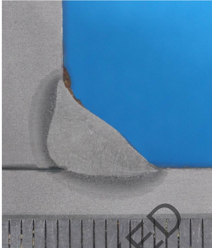
Image 1 of 2 - Macro Specimen 1 ( 1 Graduation = 1mm) M1
